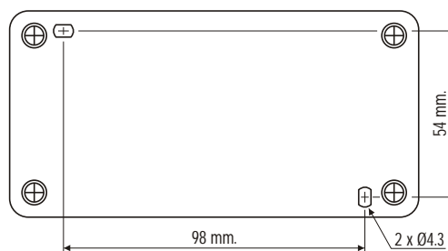
Mounting holes
